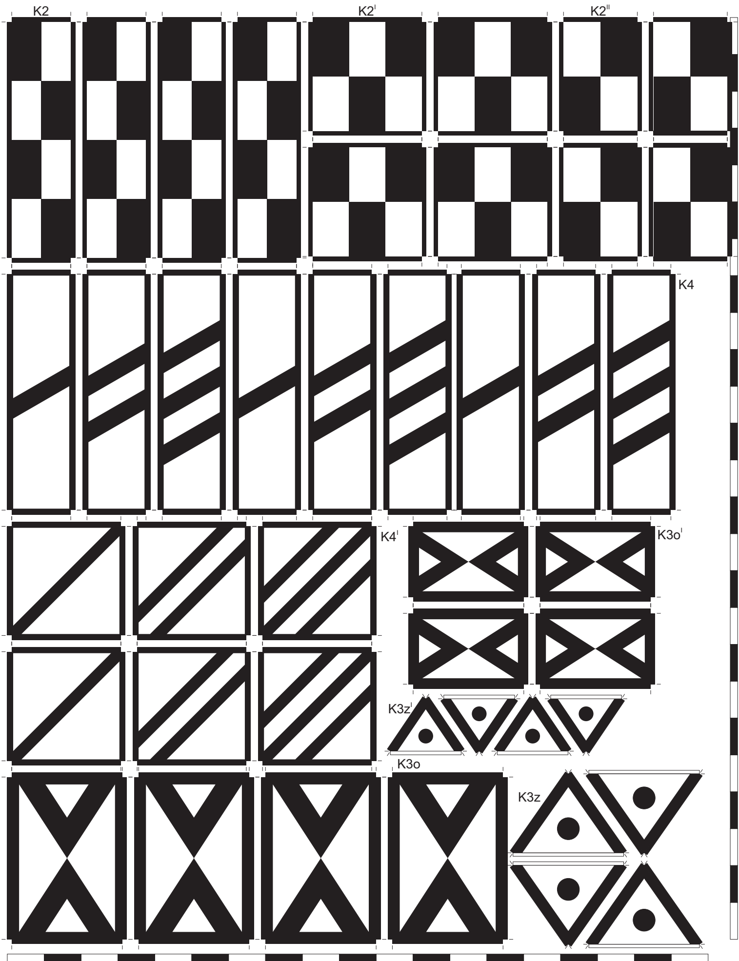
Railway signals and indicators DRG/DR, 1935-1945, scale 1:25
