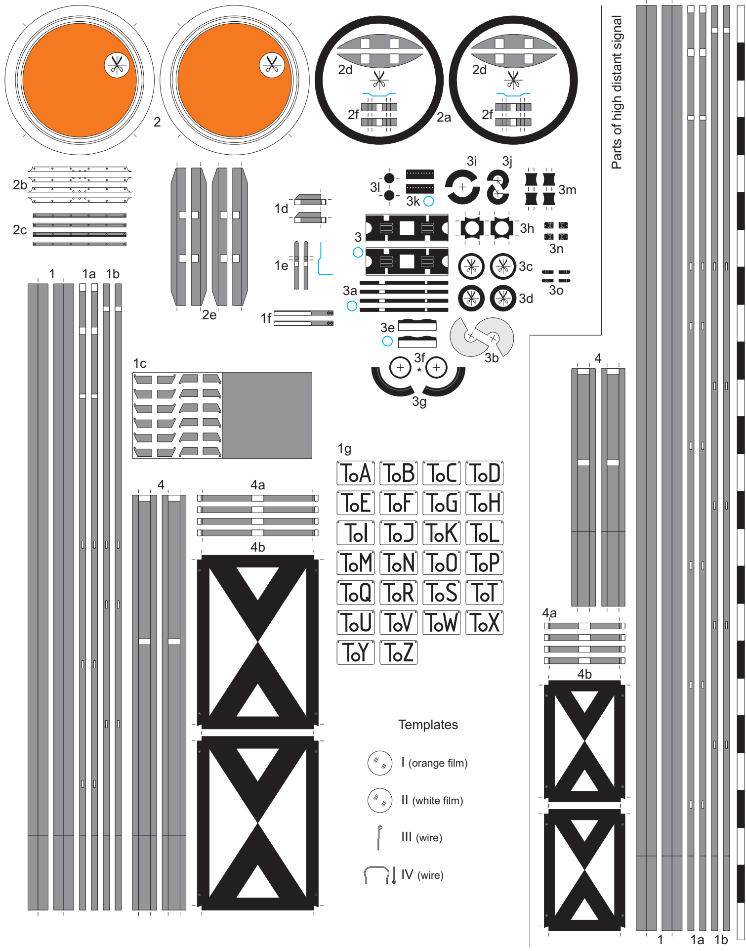
Fixed distant signal, scale 1:25
