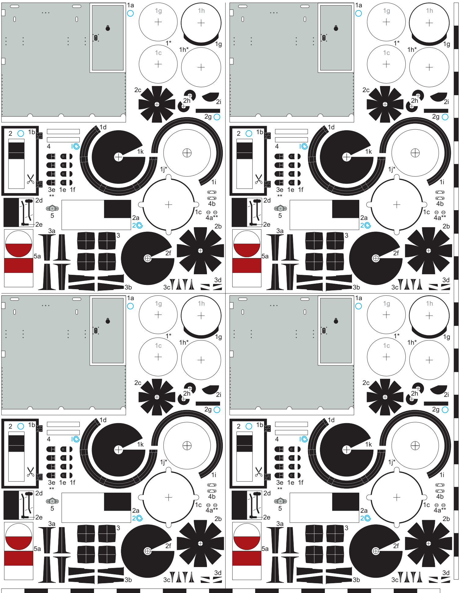
Bell signal, scale 1:35
